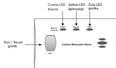
Model: K7CO
